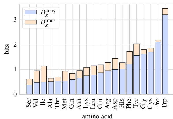
Figure 3. Copy and transformation information for different amino acids, based on an empirical PAM matrix [58]. We show magnitude of D_x^{\text{copy}}(p_{Y|x} \| p_Y) in blue; on top of this is the amount of transformation information in orange. The sum of both is the specific MI for each amino acid, according to the decomposition given in equation (2.9). (Online version in colour.)
