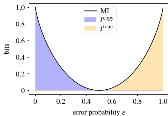
Figure 2. The binary symmetric channel (BSC) with a uniform source distribution. We plot values of the MI ( I(Y : X) ), copy information I^{\text{copy}}(X \rightarrow Y) (equation (2.10)) and transformation information I^{\text{trans}}(X \rightarrow Y) (equation (2.11)) for the BSC along the whole range of error probabilities \epsilon \in [0, 1] . When \epsilon \leq 1/2 , all mutual information is I^{\text{copy}} (blue shading); when \epsilon \geq 1/2 , all mutual information is I^{\text{trans}} (orange shading). (Online version in colour.)
